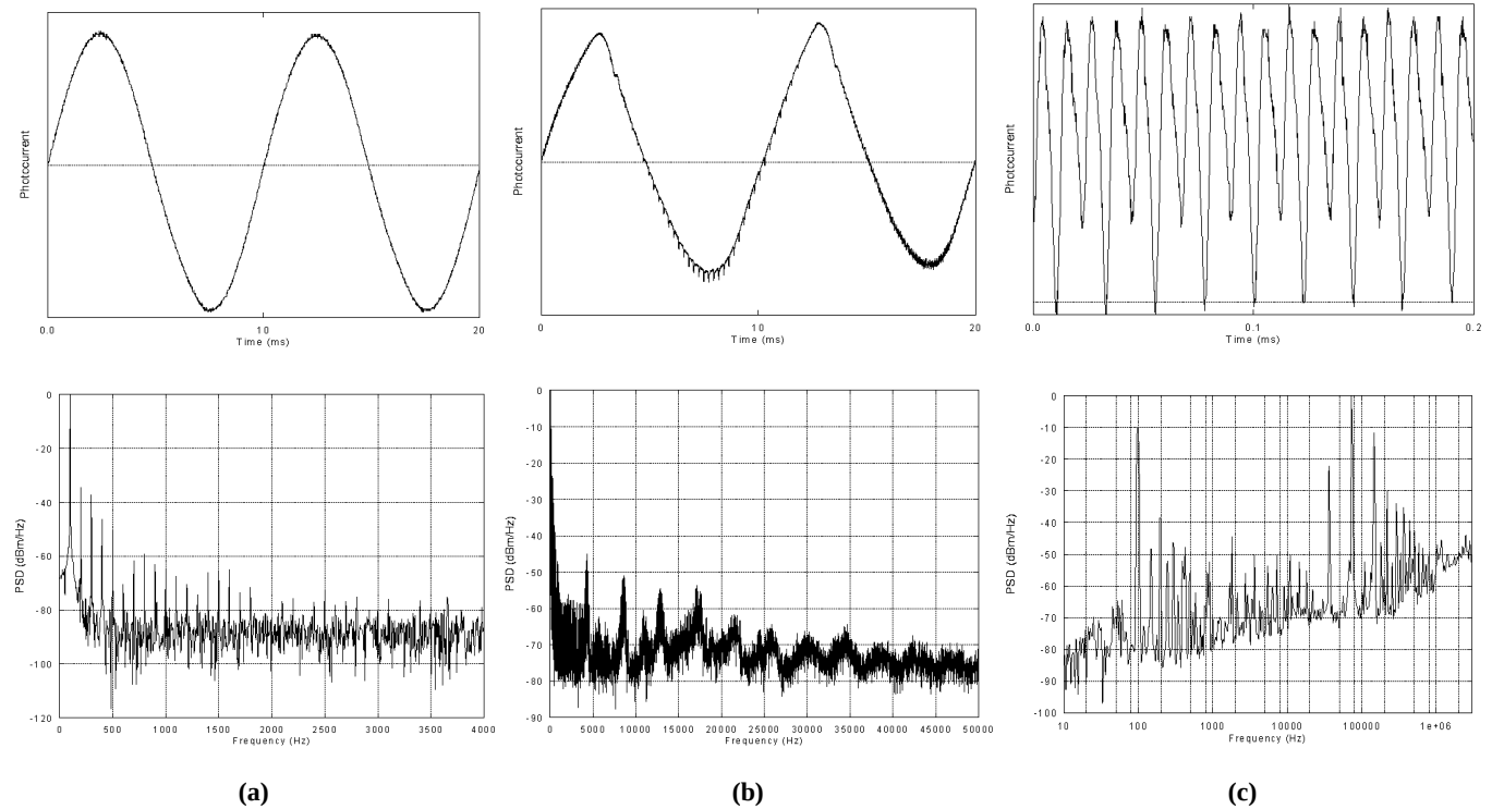
Figure 3. Photocurrent waveforms (the dc components of the waveforms was removed) and PSD:
