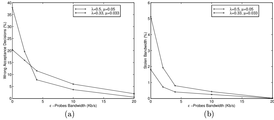
Fig. 7. Effect of time-varying offered load on (a) wrong decisions and (b) stolen bandwidth.
