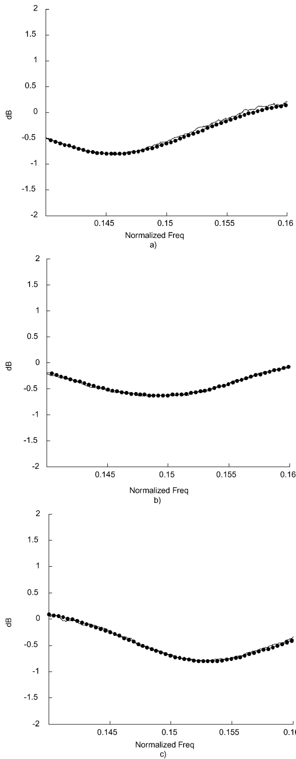
Fig. 10. In-band BLA: simulated (simple line); theoretical (dotted line). (a) Signal spectrum 1. (b) Signal spectrum 2. (c) Signal spectrum 3.
