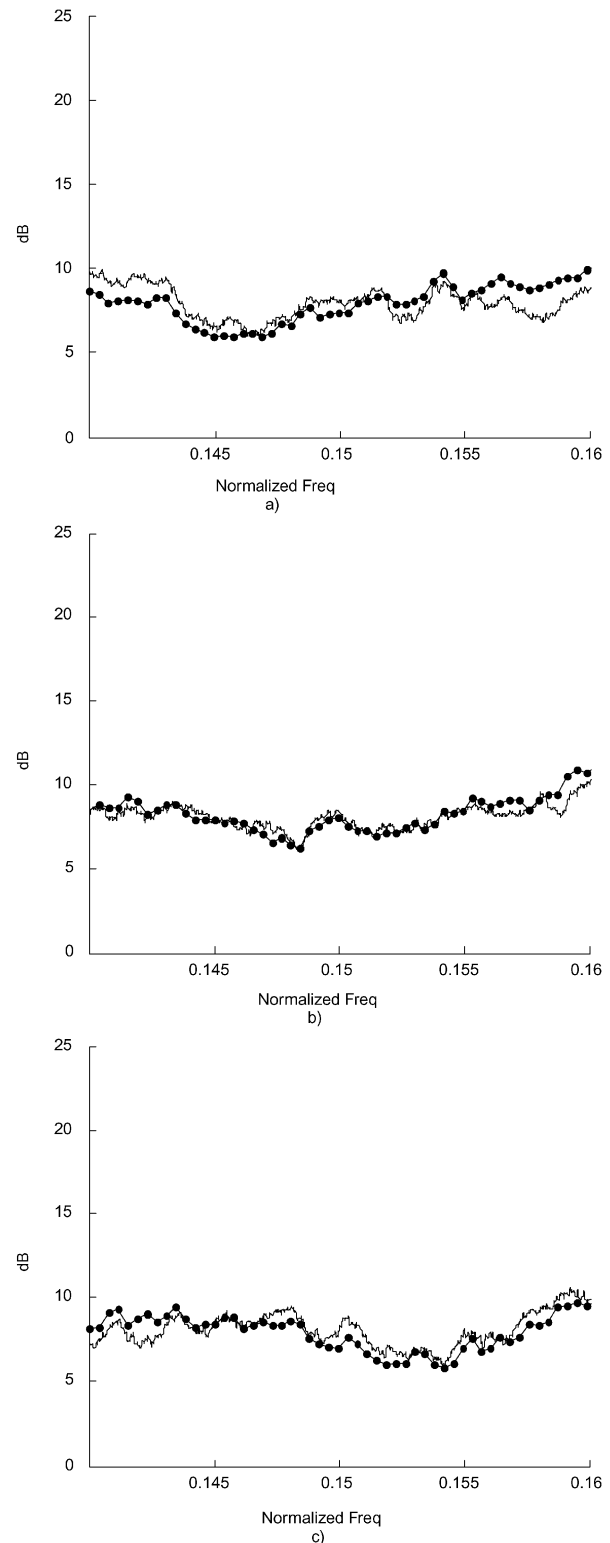
Fig. 11. In-band NDF: simulated (simple line); theoretical (dotted line). (a) Signal spectrum 1. (b) Signal spectrum 2. (c) Signal spectrum 3.
