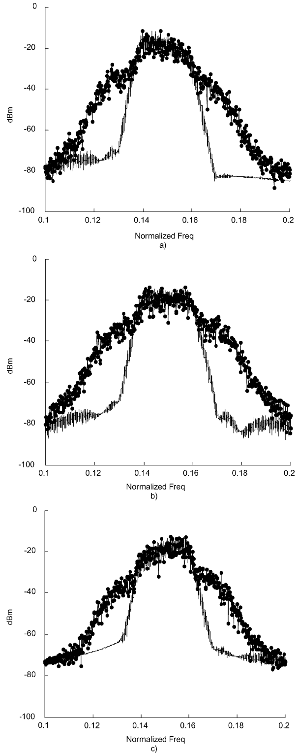
Fig. 9. Input spectrum of the test signals used for the BLA extraction (simple line) and output spectrum (dotted line). (a) Signal spectrum 1. (b) Signal spectrum 2. (c) Signal spectrum 3.
