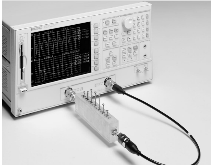
Figure 11. Eight-pole, seven-aperture filter used for Examples 2 and 3
