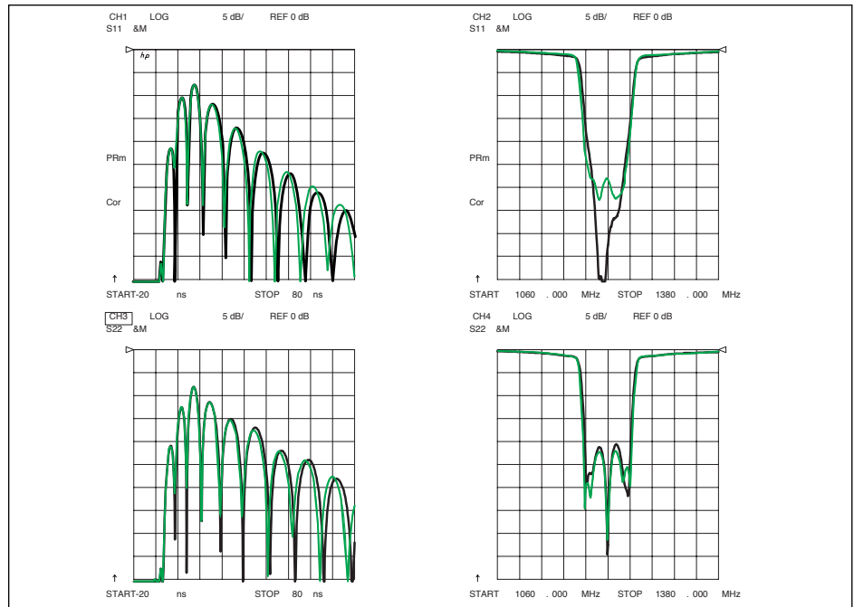
Figure 14. The response of a “golden” filter (lighter trace) and another filter with both couplings and resonators tuned (darker trace)
