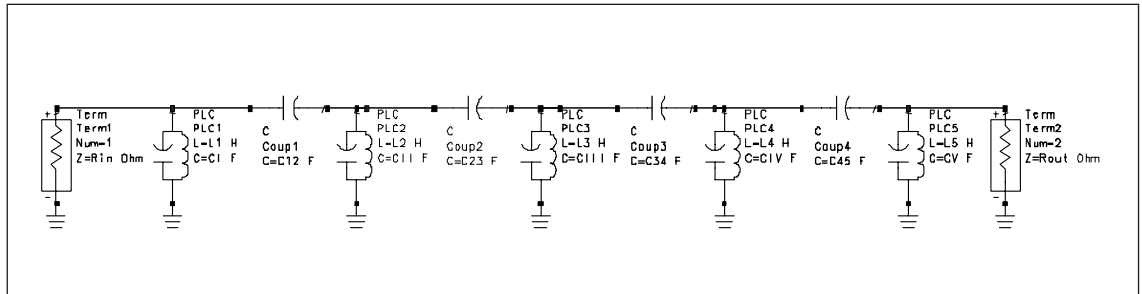
Figure 1. Schematic for five-pole coupled resonator bandpass filter
