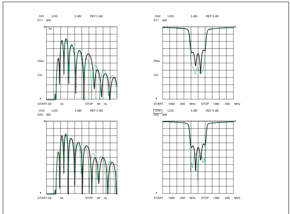
Figure 13. The response of a “golden” filter (lighter trace) and a filter where only the resonators are tuned (darker trace)
