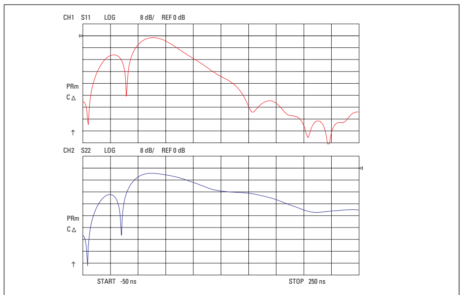
Figure 6. Time-domain response of 5-pole filter after tuning resonators 1 and 5
