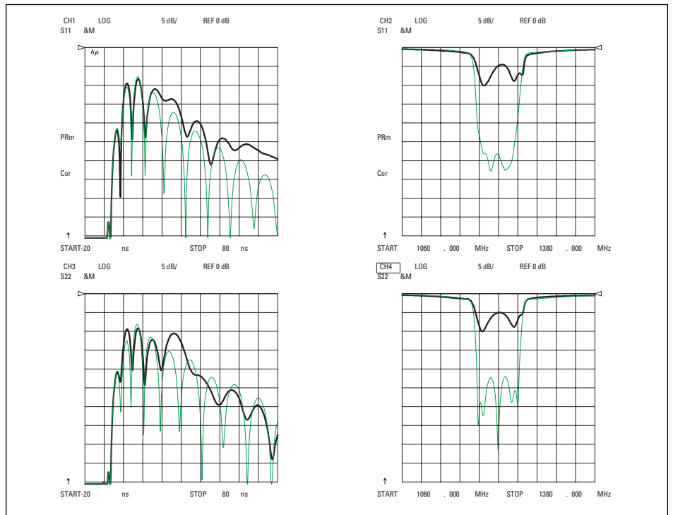
Figure 12. The response of a “golden” filter (lighter trace) and an untuned filter of the same type (darker trace)
