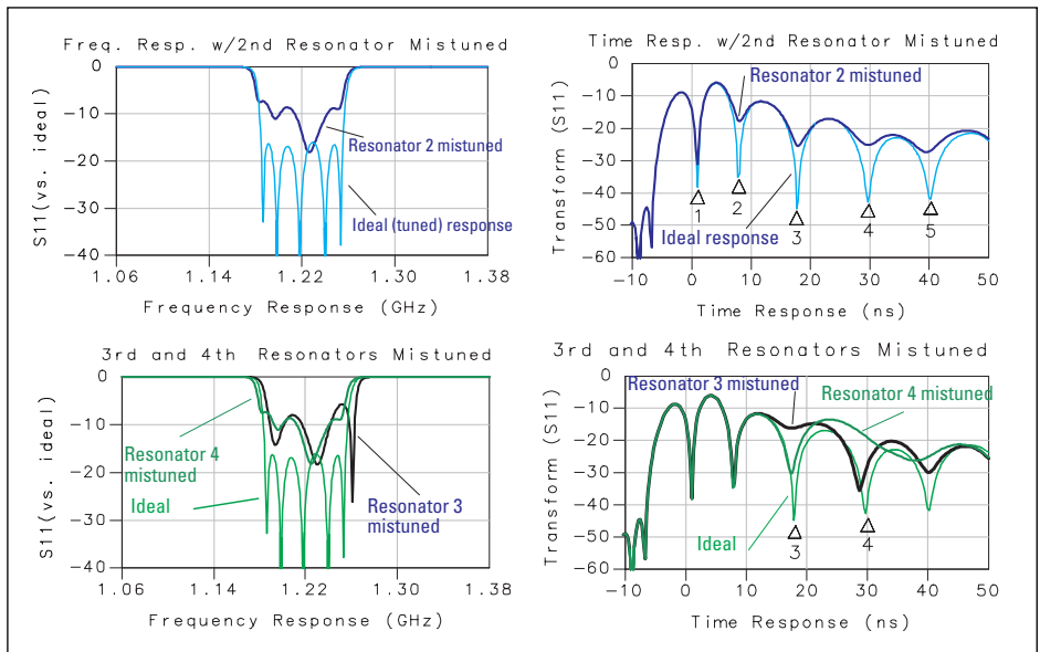
Figure 3. The response of a bandpass filter to tuning the resonators
