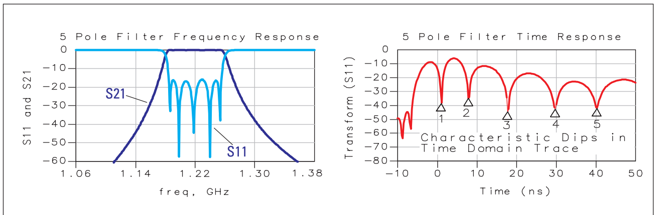
Figure 2. The frequency and time-domain response of a bandpass filter
