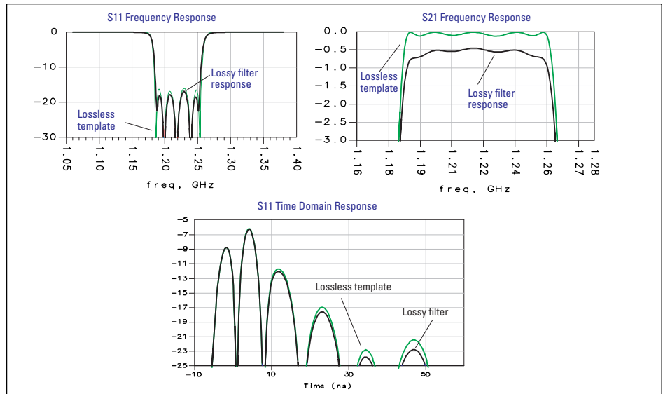
Figure 16. Comparison of lossless and lossy filters
