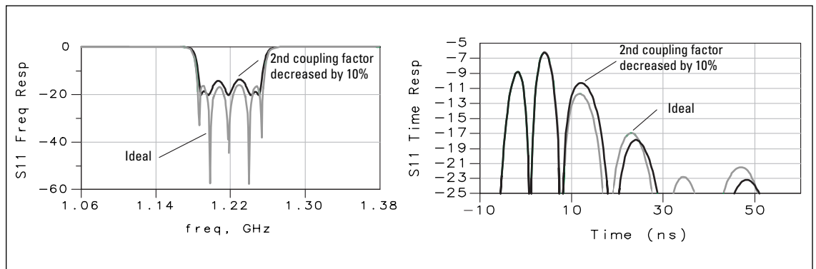
Figure 5. Effect of decreasing second coupling factor (darker trace is after adjustment)
