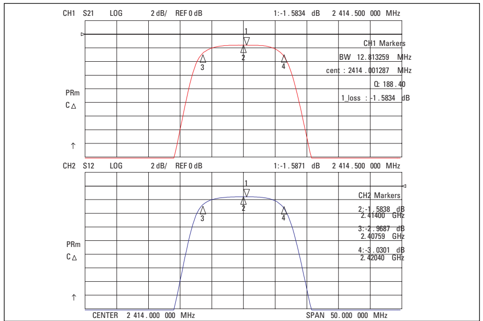
Figure 9. Final transmission frequency response
