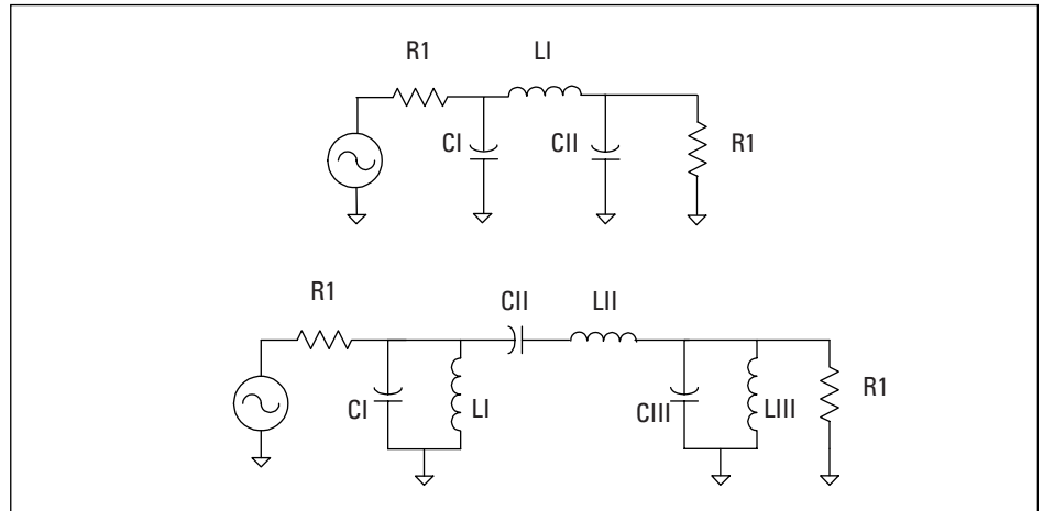
Figure 19. 3-element prototype low-pass filter and corresponding bandpass filter
