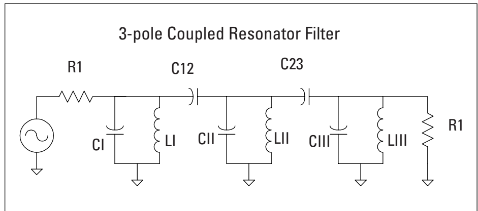
Figure 20. Equivalent 3-pole coupled resonator filter
