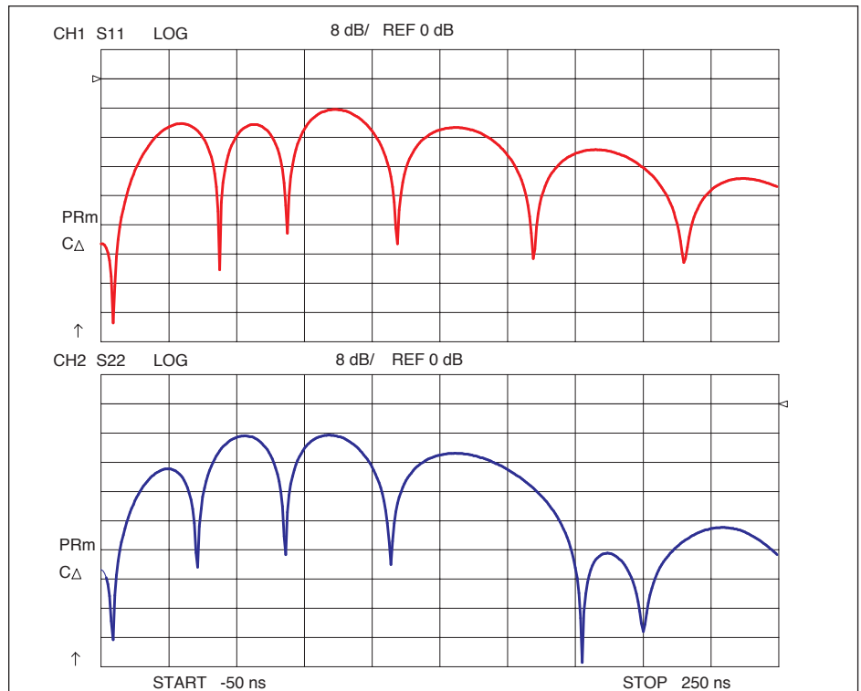
Figure 7. Time-domain response of 5-pole filter after tuning all resonators
