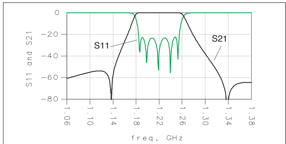
Figure 17. Transmission and reflection responses of a filter with symmetrical transmission zeros
