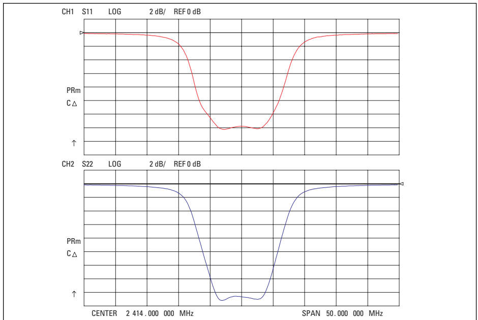
Figure 8. Final reflection frequency response
