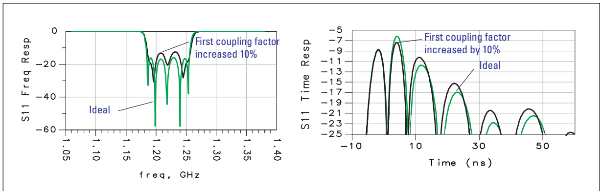
Figure 4. Effect of increasing first coupling factor (darker trace is after adjustment)
