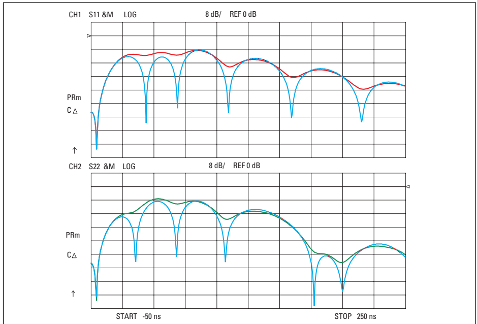
Figure 10. Time-domain response with center frequency changed
