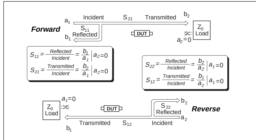
Figure 17. Measuring S-Parameters
