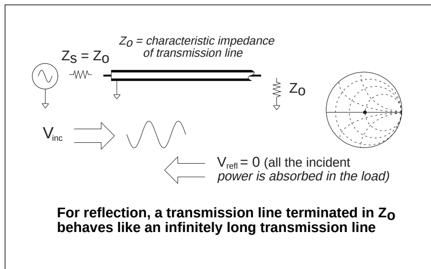
Figure 8. Transmission Line Terminated with Z_0
