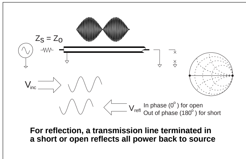
Figure 9. Transmission Line Terminated with Short, Open
