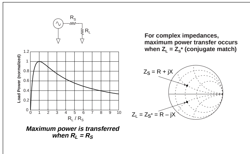
Figure 7. Power Transfer
