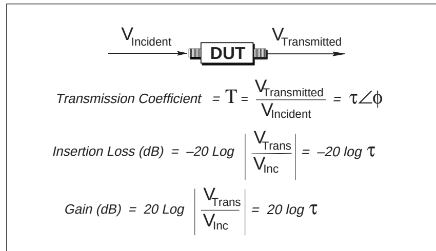
Figure 12. Transmission Parameters
