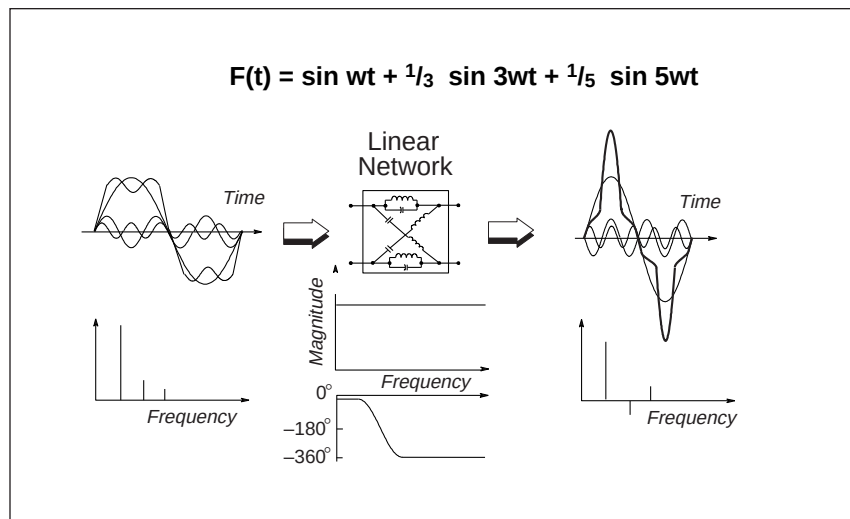
Figure 3. Phase Variation with Frequency
