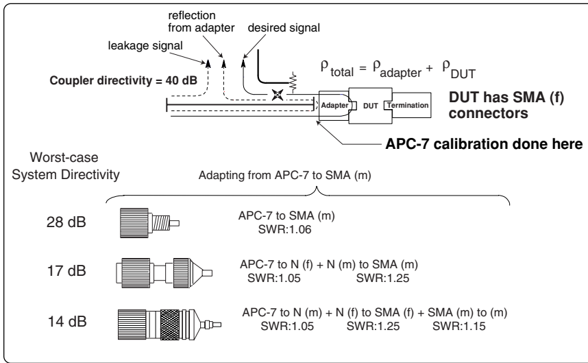
Figure 4. Adapter Considerations
