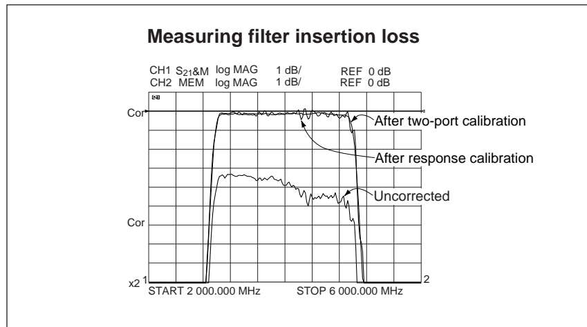
Figure 1. Response versus Two-Port Calibration
