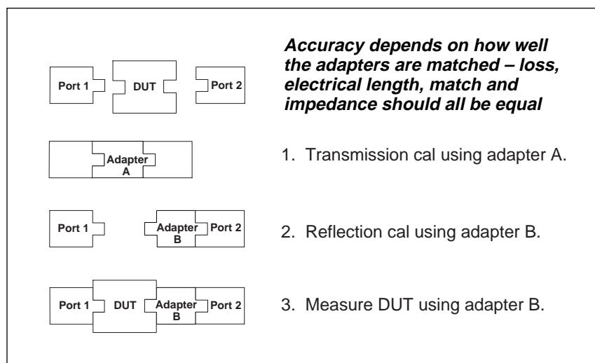
Figure 15. Swap-Equal-Adapters Method
