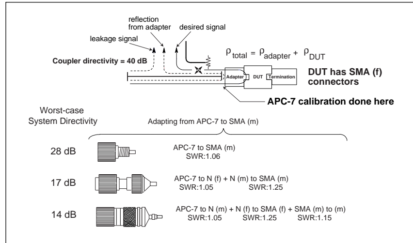
Figure 4. Adapter Considerations
