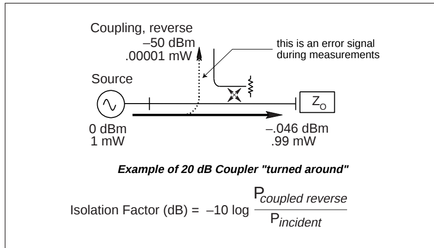
Figure 4. Directional Coupler Isolation (Reverse Coupling Factor)
