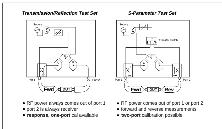
Figure 9. T/R versus S-Parameter Test Sets
