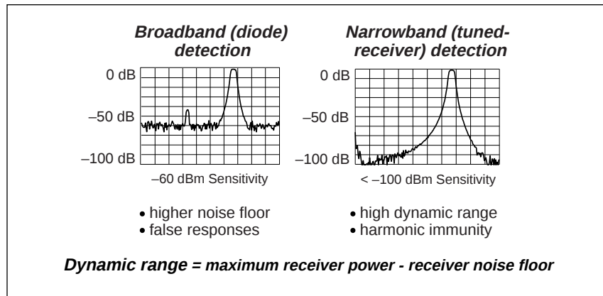
Figure 7. Comparison of Receiver Techniques
