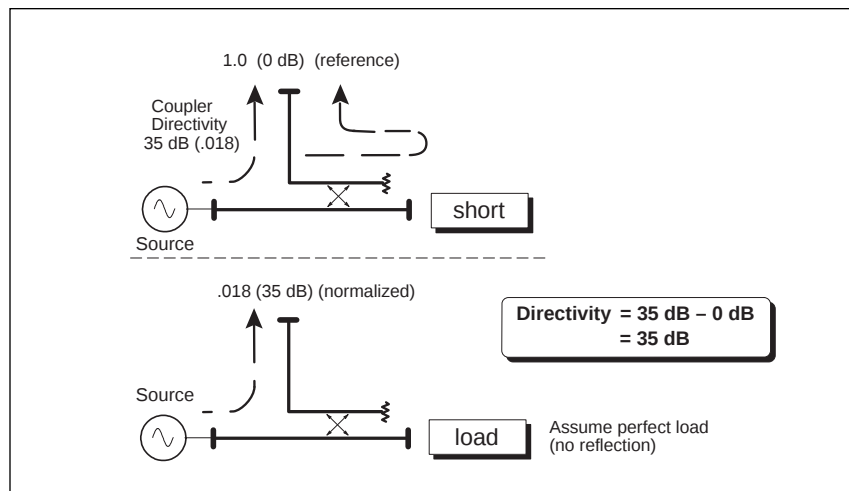
Figure 6. Measuring Directivity the Easy Way
