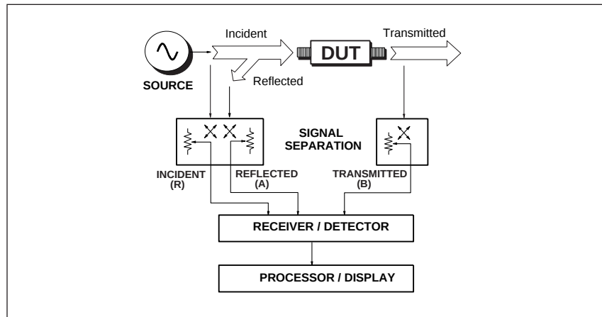
Figure 2. Generalized Network Analyzer Block Diagram
