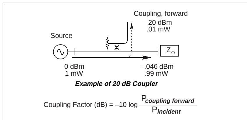
Figure 3. Forward Coupling Factor
