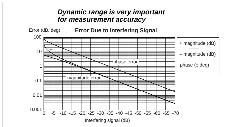
Figure 8. Dynamic Range and Accuracy
